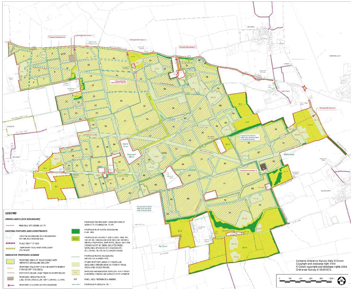
Plate 5-1 Indicative Site Layout Plan
